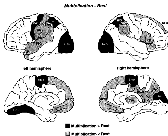
Fig. 3. Schematic representation of the regions of interest that were significantly activated or deactivated during multiplication relative to rest, as projected on a lateral and mesial view of the two hemispheres. Abbreviations: LOC, lateral occipital cortex; PrG, precentral gyrus; SMA, supplementary motor area; PoG, postcentral gyrus; SmG, supramarginal gyrus; IFG, inferior frontal gyrus; Tha, thalamus; STG, superior temporal gyrus; Cu, cuneus; FLG, fusiform and lingual gyri; IPG, inferior parietal gyrus; PrC, precuneus; TP, temporal pole; SFG, superior frontal gyrus; MPfC, medial prefrontal cortex; PoC, posterior cingulate gyrus.
