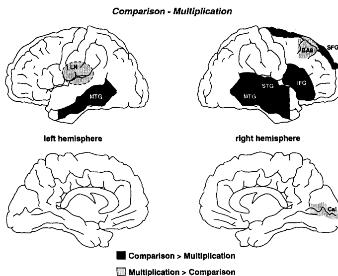
Fig. 4. Schematic representation of the regions of interest that were differentially activated during comparison and during multiplication, as projected on a lateral and mesial view of the two hemispheres. Abbreviations: BA8, Brodmann's area 8; STG, superior temporal gyrus; MTG, middle temporal gyrus; IFG, inferior frontal gyrus; SFG, superior frontal gyrus; Cal, calcarine cortex.
